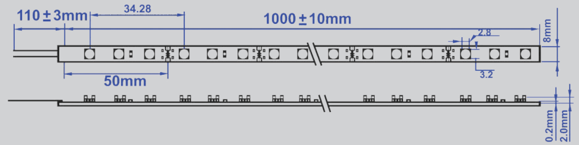
Şerit Led Detay Led Strip Detail
