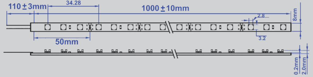
Şerit Led Detay Led Strip Detail
