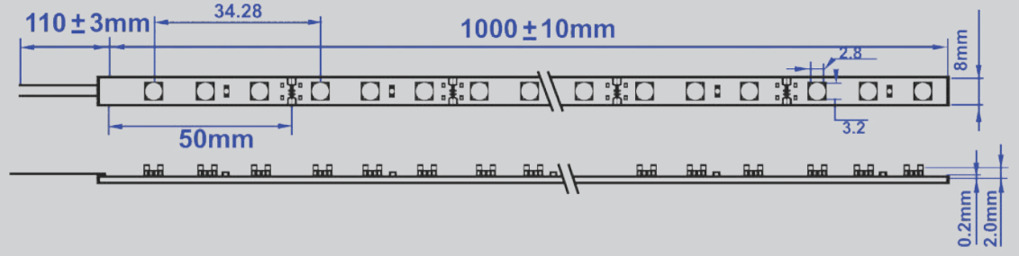
Şerit Led Detay Led Strip Detail
