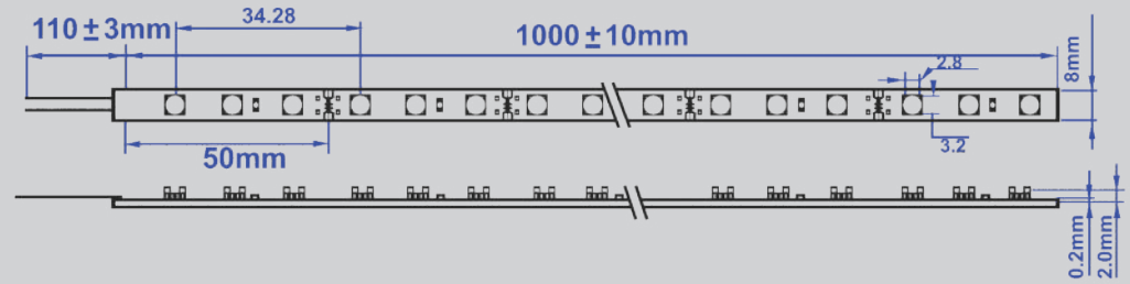
Şerit Led Detay Led Strip Detail
